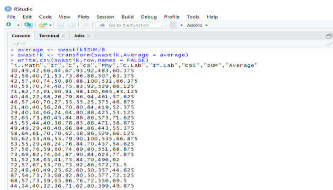
Figure 3: Perform Average operation in CSV
