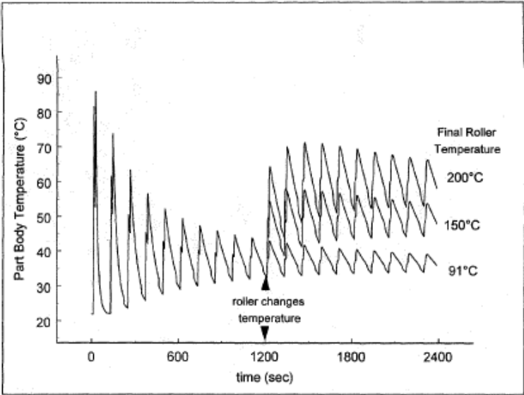
Figure 6: Effect of changing the roller temperature (from 91°C) halfway through a run: simulated, dynamic temperature profiles inside a 20-layer SiC LOM part during the building process (120 seconds per layer) using the parameters given in Table 2 (trials 17, 18).
