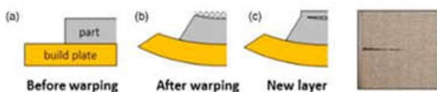
Figure 7: Schematic of build plate warping effect during processing (a-c) and resultant damage
