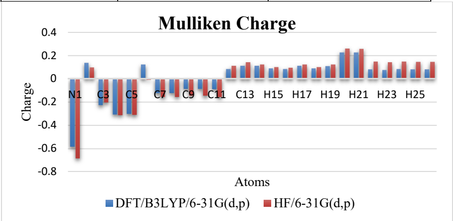
Fig.6. Muliken’s atomic charges of 2-methyl-1phenylpropan-2-amine
